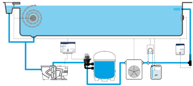
TYPICAL SALT INSTALLATION
