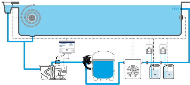
TYPICAL CHLORINE INSTALLATION
